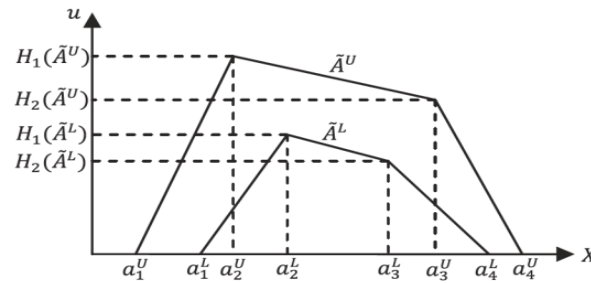
Figure.1. A trapezoidal interval type-2 fuzzy set A^{\perp \approx} (Chen & Lee, 2010b)
